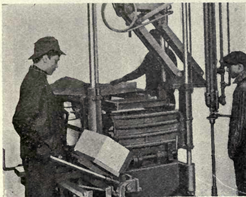
FIG. 14—DETAIL VIEW OF HYDRAULIC PRESSURE MACHINE
